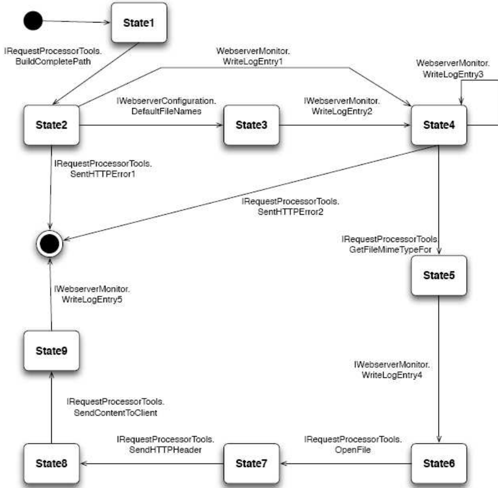
Fig. 4. IHTTPRequestProcessor.HandleRequest: Service Effect Automaton
