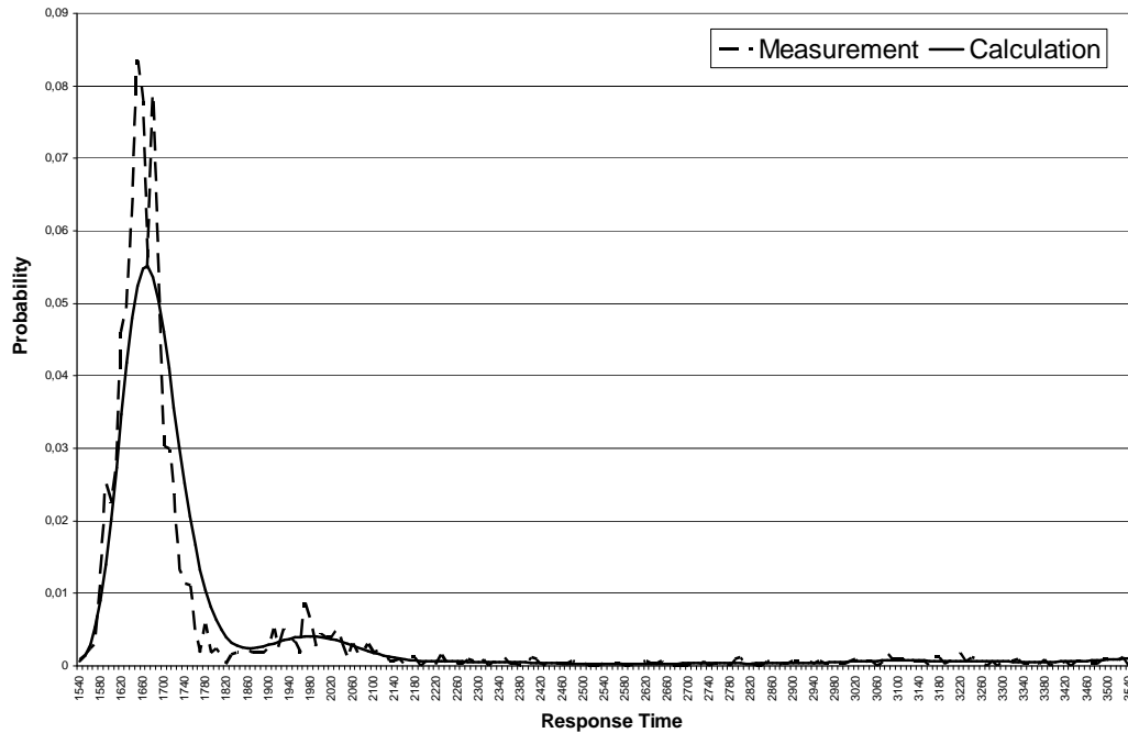
Fig. 9. Scenario 1 (Sequence): Probability Mass Functions
